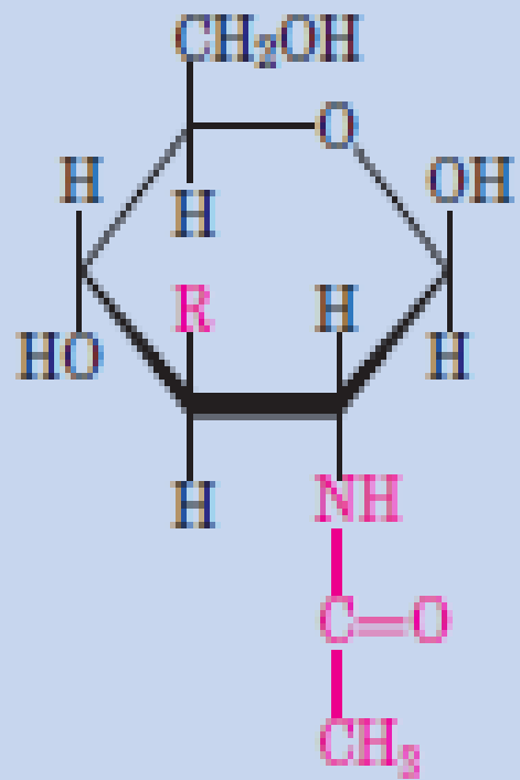
N-Acetylmuramic acid
