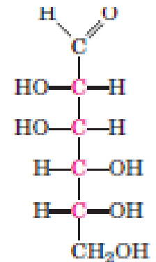
D-Mannose
