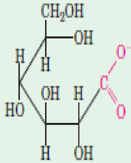
D-Gluconate
