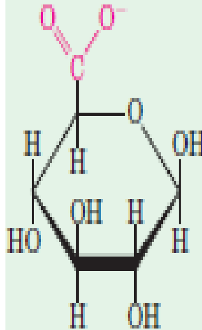
\beta -D-Glucuronate
